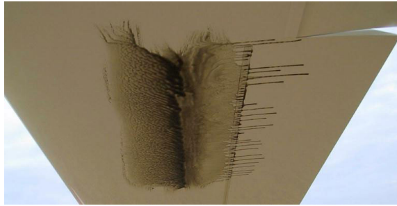
Figure 13: Normal Lower Surface Oil-Flow Image
