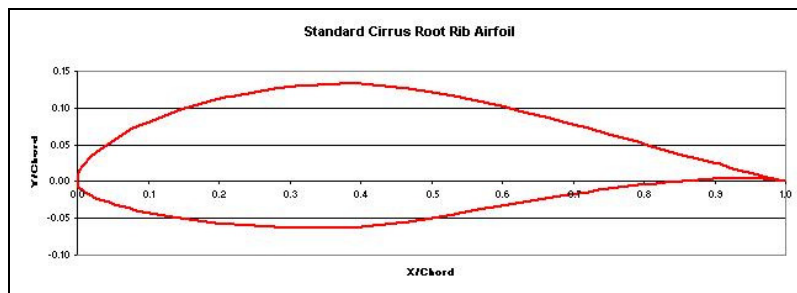
Figure 2: FX S 02-196 Standard Cirrus Root Airfoil
